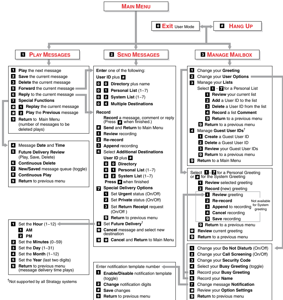
Figure 1 Strategy Main Menu
